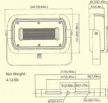
45W( Trunnion Mount)
