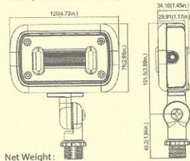
15W( Knuckle Mount)
