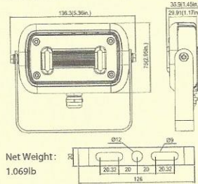
30W( Trunnion Mount)
