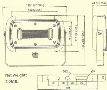
30W( Trunnion Mount)
