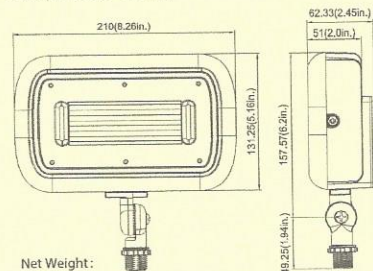
45W( Knuckle Mount)
