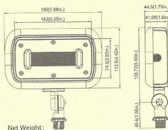
30W( Knuckle Mount)
